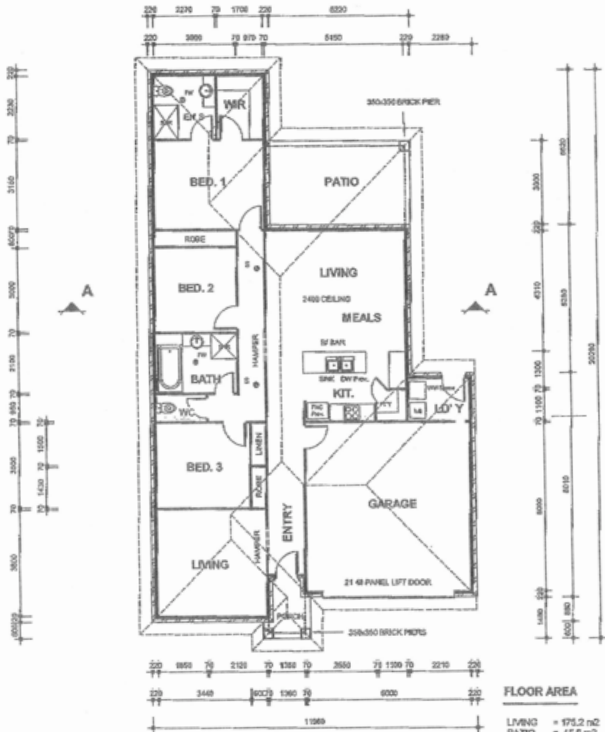
FLOOR PLAN 1:100
